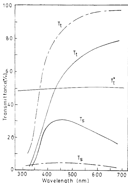
Figure 6. Total ( T_t ) and scattered ( T_s ) transmittance of 2-mm-thick specimen. Solid line represents dry stage; dash-dot line represents water-impregnated condition. Also shown is T_t of a dense transparent commercial alumina. Reprinted with permission from ref 89; copyright 1975 Americal Ceramic Society.
