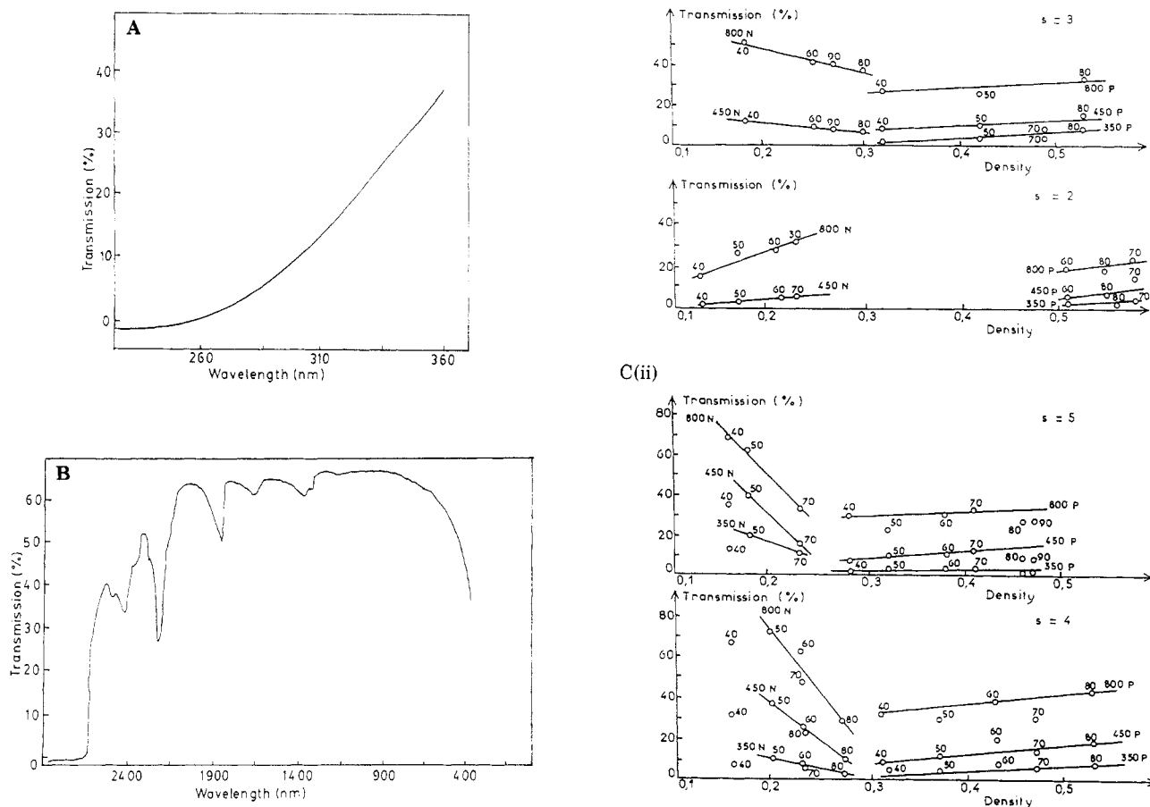
Figure 2. (A) UV transmission of a silica aerogel (density 0.16 g/mL) of 0.4-mm thickness. (B) Visible and near-IR transmission of a silica aerogel (density of 0.16 g/mL) of 0.4-mm thickness. (C) Transmission of silica aerogels at three wavelengths, 350, 450, and 800 nm, as a function of S , the ratio of moles of water to moles of methyl orthosilicate, and the resultant density. Hydrolysis conditions: N = ammonia; P = neutral. (i) For S = 2 and 3; (ii) for S = 4 and 5. Reprinted with permission from ref 18; copyright 1977, University Claude Bernard, Lyon.
